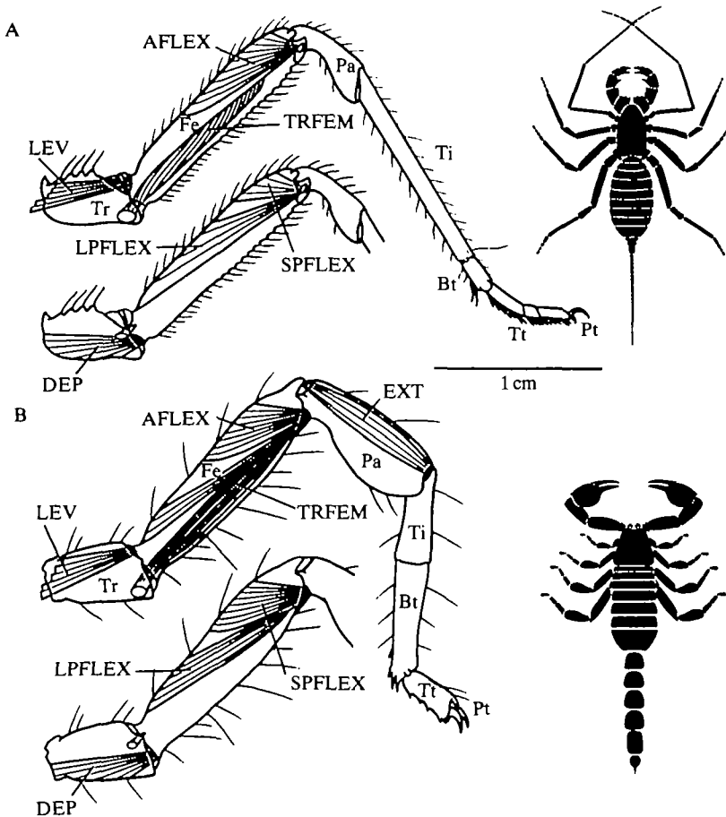
Fig. 1. Skeletomuscular anatomy of walking legs in (A) the giant whisperscorpion Mastigoproctus giganteus (Uropygi) and (B) the black emperor scorpion Pandinus imperator (Scorpiones). Upper diagrams depict an anterior/lateral view of the fourth walking leg from the left side of the body. Lower diagrams depict posterior muscles with anterior muscles removed. AFLEX, anterior flexor; Bt, basitarsus; DEP, depressor; EXT, extensor; Fe, femur; LEV, levator; LPFLEX, long posterior flexor; Pa, patella; Pt, pretarsus (apotele); SPFLEX, short posterior flexor; Ti, tibia; Tr, trochanter; TRFEM, transfemoral muscle; Tt, telotarsus.
