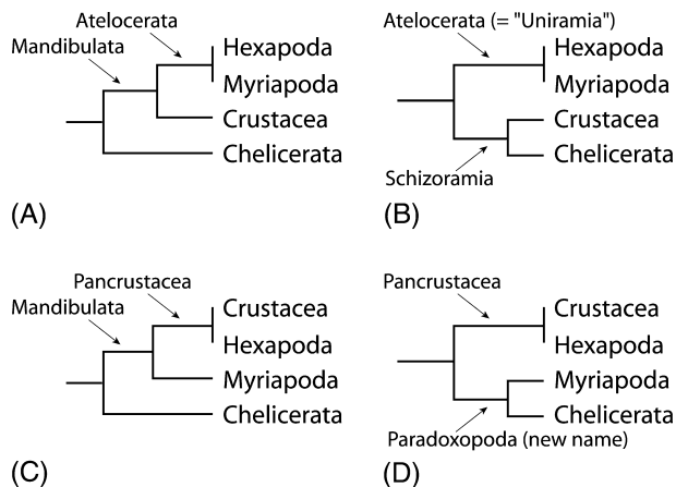
Fig. 1. Major hypotheses of the relationships of arthropod groups: (A) classical 'Mandibulata' (= Mandibulata + Chelicerata), in which the three groups possessing mandibles formed by the second post-oral appendage (hexapods, myriapods, crustaceans) are distinguished from chelicerates; (B) Atelocerata versus Schizoramia: clades with unbranched versus two-branched appendages; (C) Pancrustacea + Myriapods within Mandibulata: that is, in the Mandibulata, hexapods group with crustaceans instead of with myriapods; (D) 'Chelicerata + Myriapoda' versus 'Crustacea + Hexapoda.'
